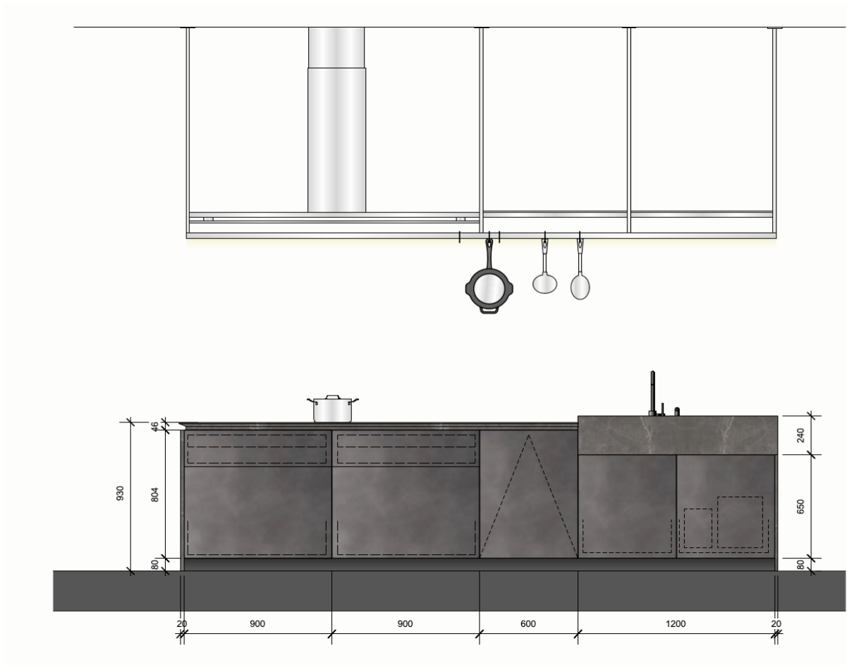
VIEW B
